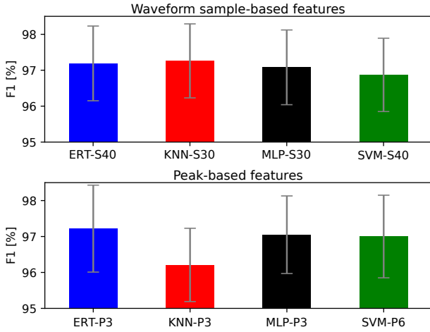
Figure 4: Comparison of classifiers' performance on the cross-validation dataset for sample-based (top) and peak-based features (bottom) in terms of F1 and 95% confidence intervals. CLF- S_n and CLF- P_m denote the classifier type (CLF), the number of samples corresponding to a window of length n ms ( S_n ), and the number of peaks prior and subsequent to a given peak ( P_m ).
